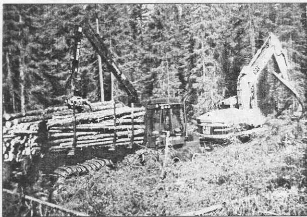
Figure 5. A Timberjack 1210 forwarder and a Caterpillar 320 harvester equipped with a Keto 150 harvesting head were used in the trials.
