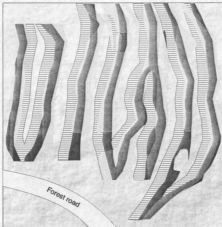
Figure 2. A cutover in which cut-to-length harvesting was conducted (in the Ashuapmushuan Wildlife Reserve in Quebec, 1993).
